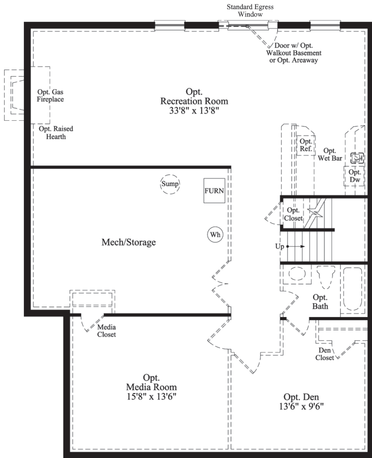
Lower Level w/ Elev. 1, 2 & 3
