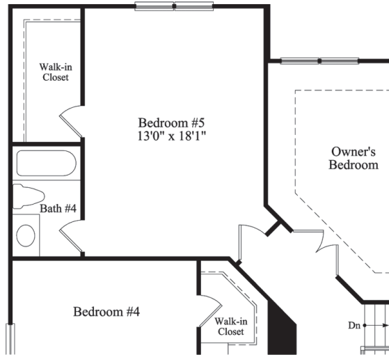
Opt. Bedroom #5 w/ 4'-0" Extension
